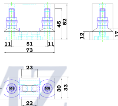
CIP100200100 = Modular fuse holder for Mega-fuse
